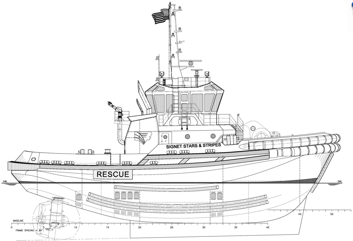
Profile View
