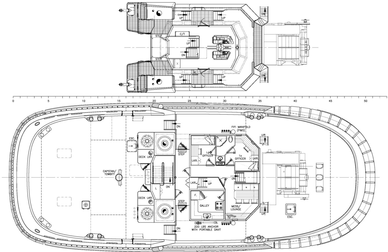
Plan View
